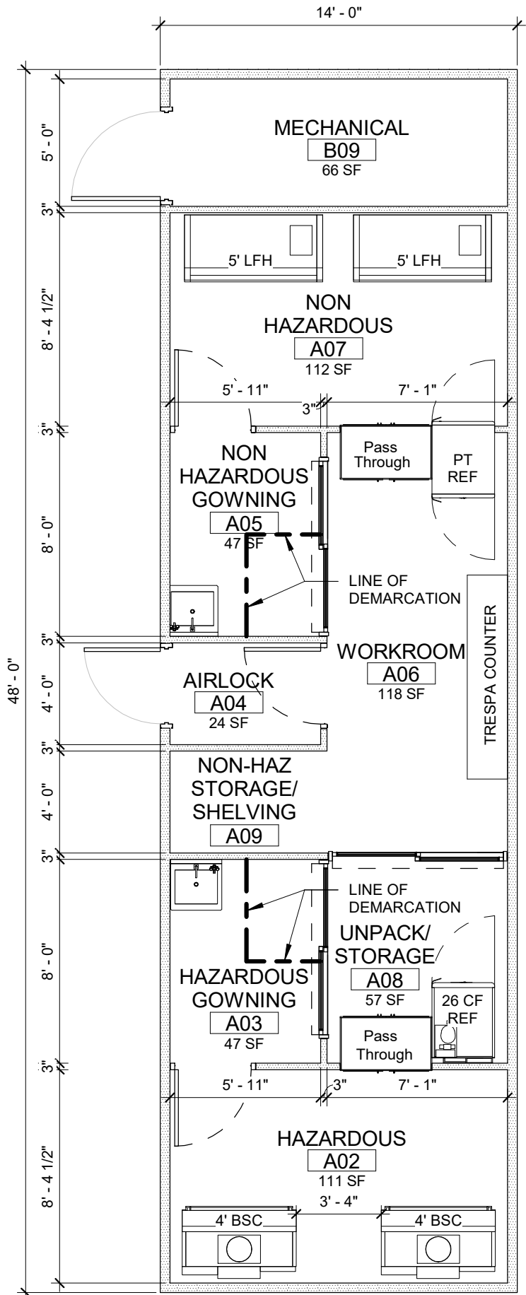
PHARMACY CLEANROOM CONCEPT
